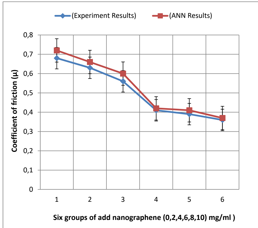
Fig. 18 Effect the concentration of nano graphene on COF.
