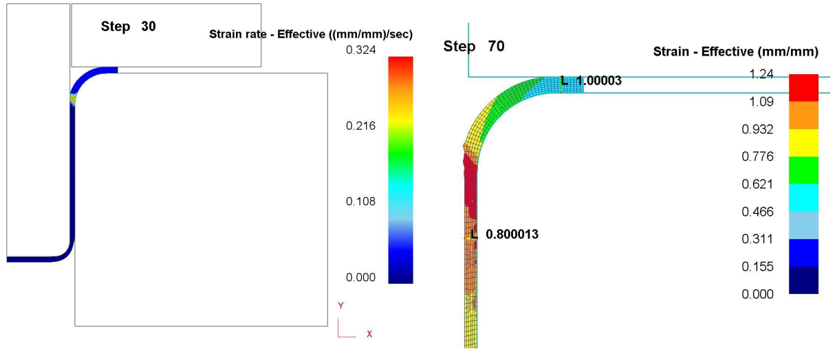
Fig. 13 Contour plots for different distributions and conditions for deep drawing die.
