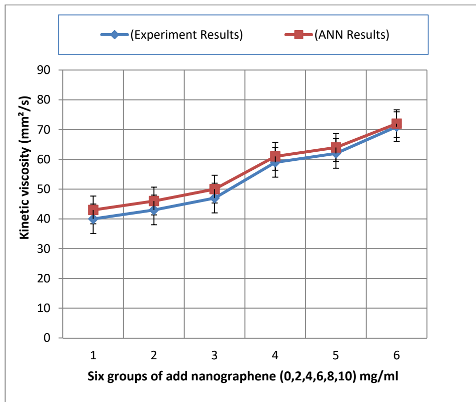
Fig. 19 Effect of concentration of nano graphene on kinetic viscosity of oil.
