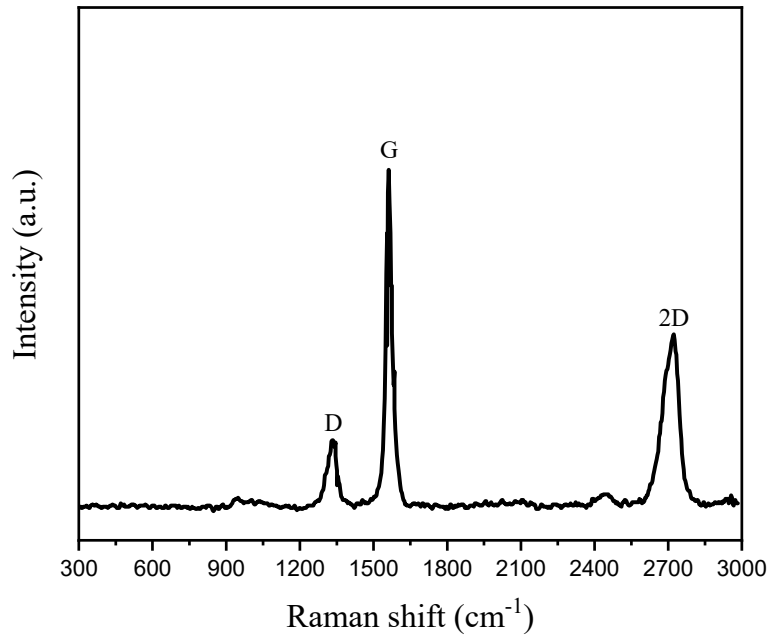
Fig. 5 Raman-spectra of graphene particles [7].
