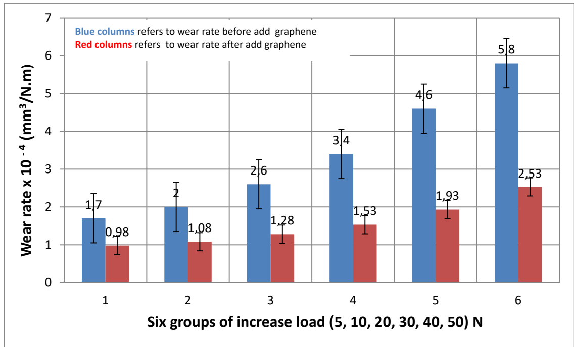
Fig. 23 Results compare of wear rate between before and after addition nano-graphene, when raised the load.
