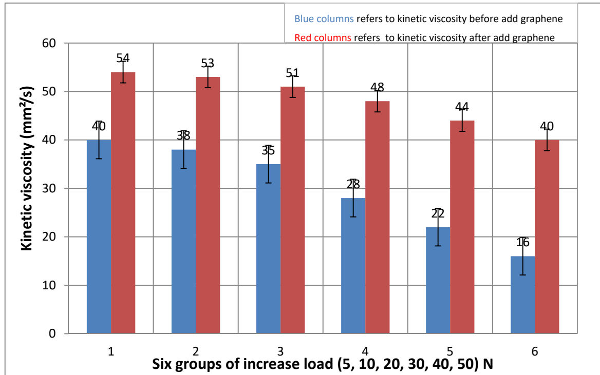
Fig. 25 Results compare of kinetic viscosity between before and after addition nano-graphene, when raised the load.
