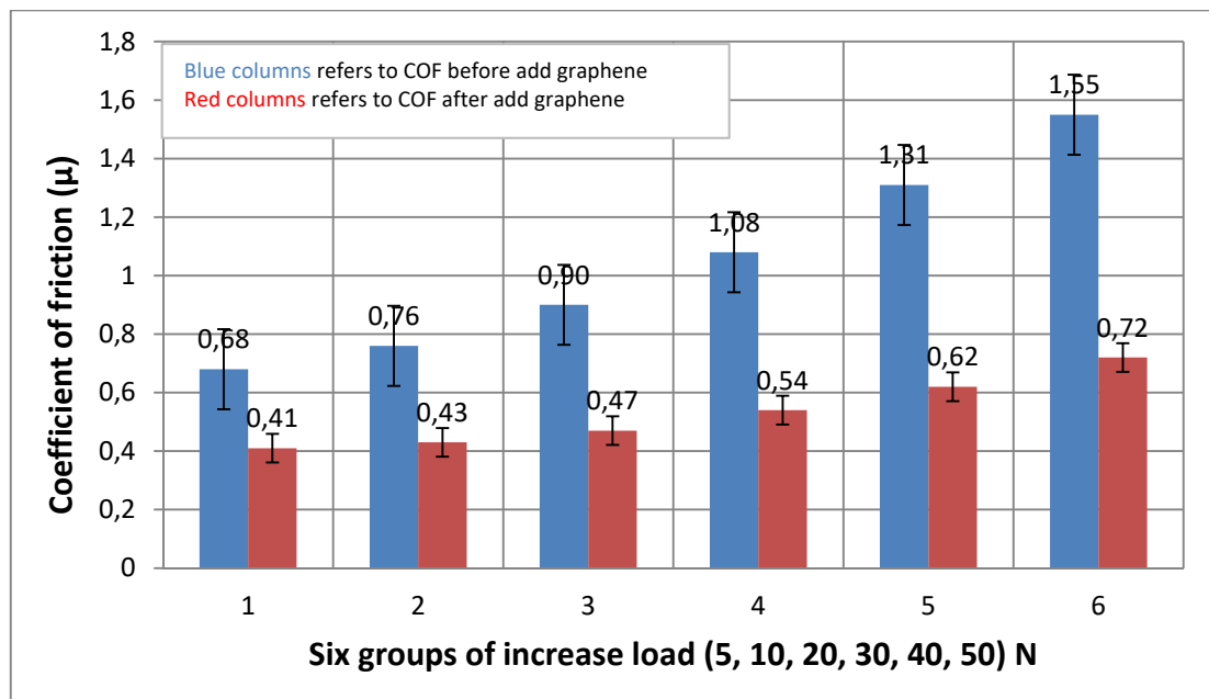
Fig. 24 Results compare friction coefficient between before and after addition nano-graphene, when raised the load.
