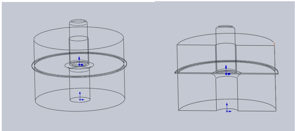
Fig. 2 Design deep drawing dies and estimate perfect stress-effective by 3D deform.
