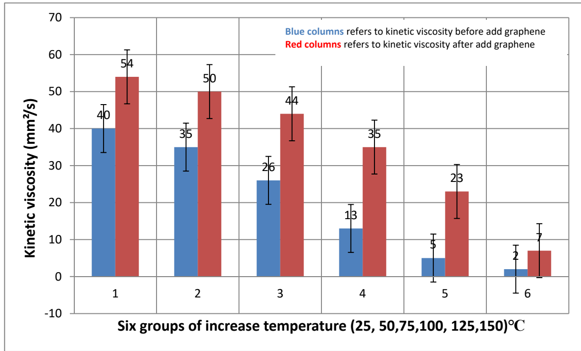
Fig. 22 Results compare kinetic viscosity between before and after addition nano-graphene, when raised the temperature.
