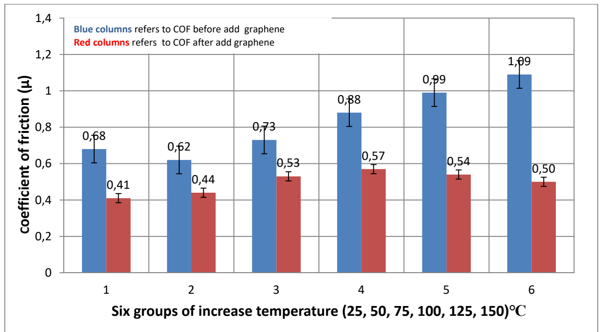
Fig. 21 Results compare friction coefficient between before and after addition nano-graphene, when raised the temperature.
