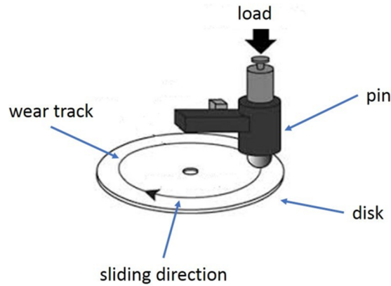
Fig. 6 Pin on disk experiment.
