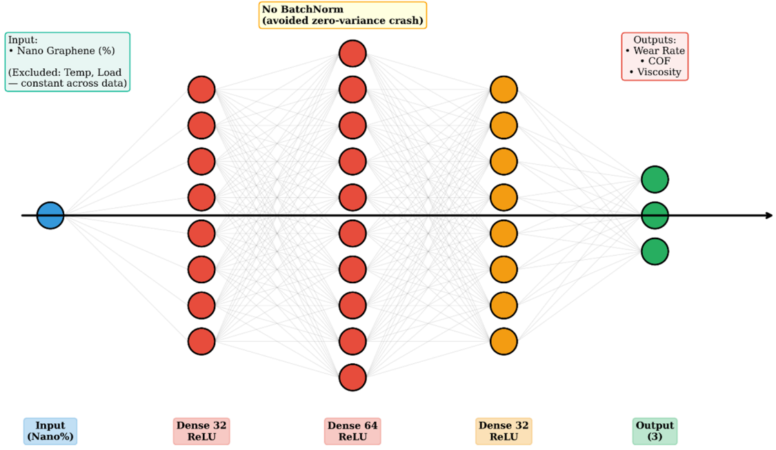
Fig. 9 Proposed DNN architecture
