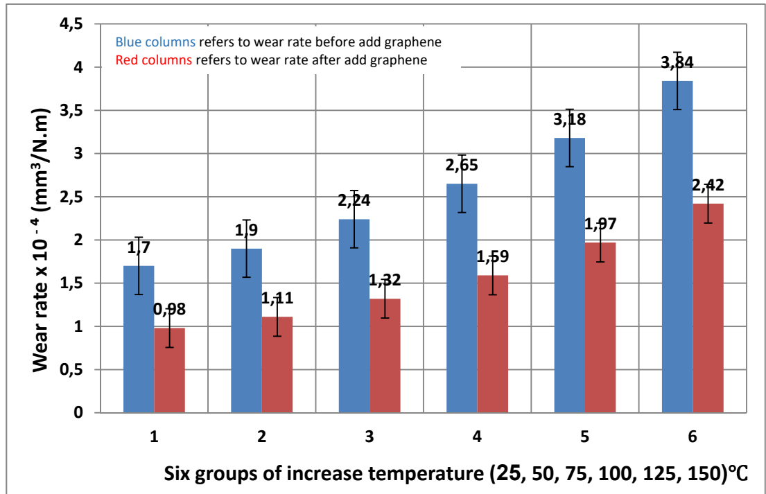
Fig. 20 Results compare of wear rate between before and after addition nano-graphene, when the temperature rose.
