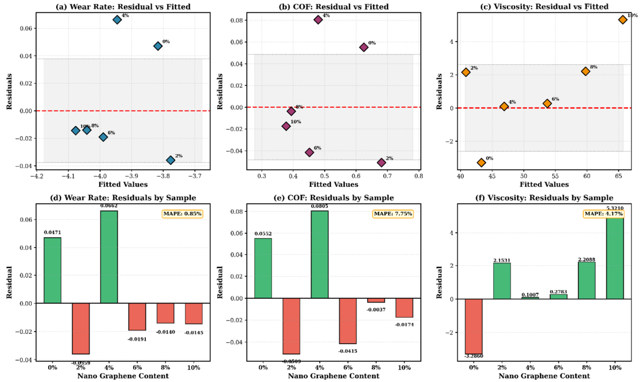
Fig. 12 LOOCV Residual Analysis
