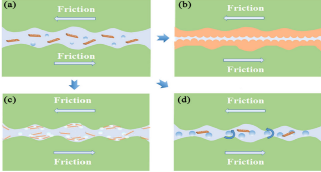
Fig. 8 Schematic illustration of lubrication mechanisms of graphene-based nanomaterial additives: a) Initial state; b) Forming tribofilm; c) Self-repairing; d) Rolling bearing.
