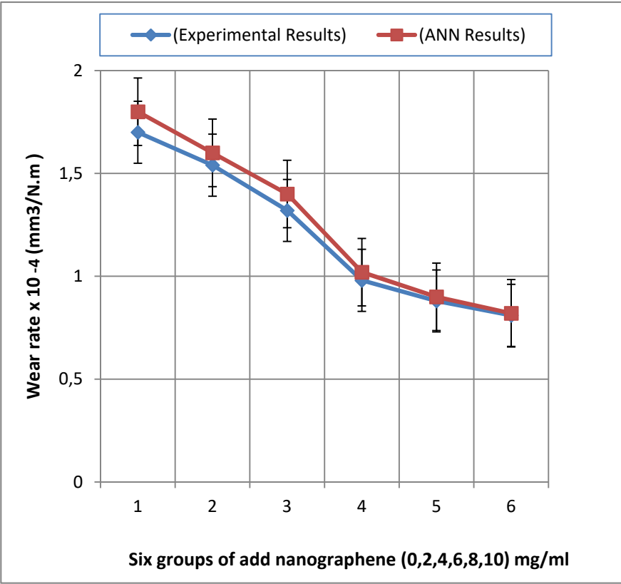
Fig. 17 Effect the concentration of nano graphene on wear rate.
