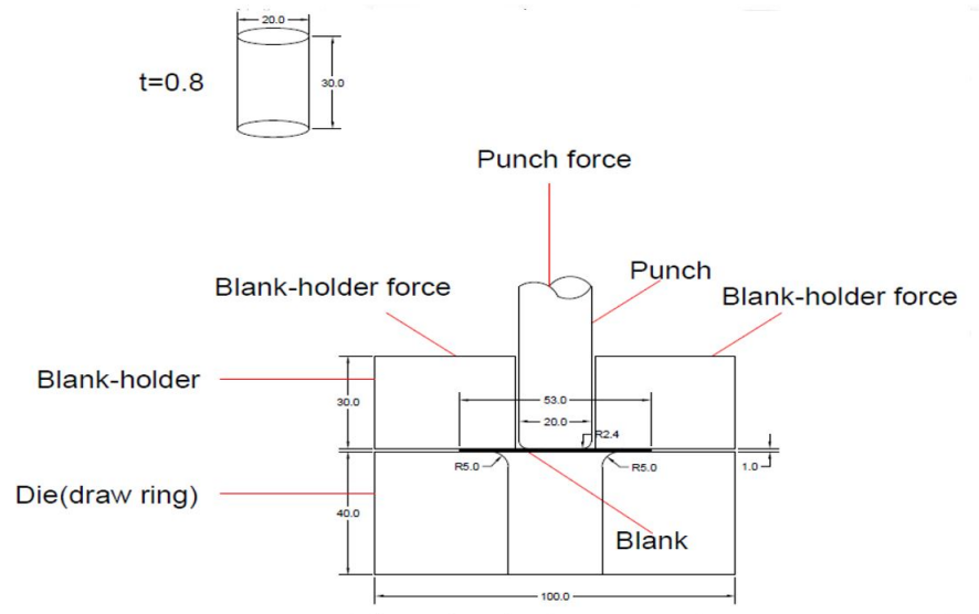
Fig. 1 Design parts of deep drawing dies and dimension.
