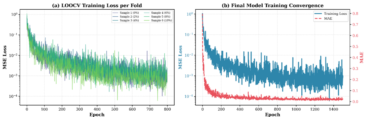
Fig. 10 Model Training Dynamics
