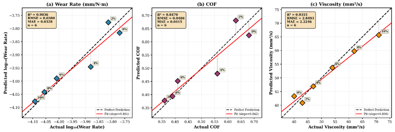
Fig. 11 Leave-One-Out Cross-Validation Parity Plots
