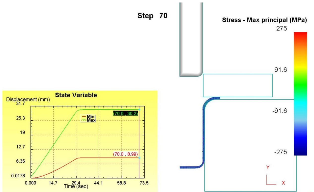
Fig. 16 Displacement contour plot during the deep drawing process.
