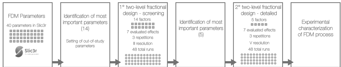
Fig. 1 Recommended FDM characterization procedure
