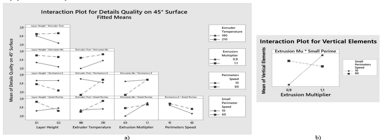
Fig. 4 a) Interaction Plot for Details Quality for the 45° surface; b) Interaction Plot for the Vertical Elements, limited to the Extrusion Multiplier/Small Perimeters Speed interaction
