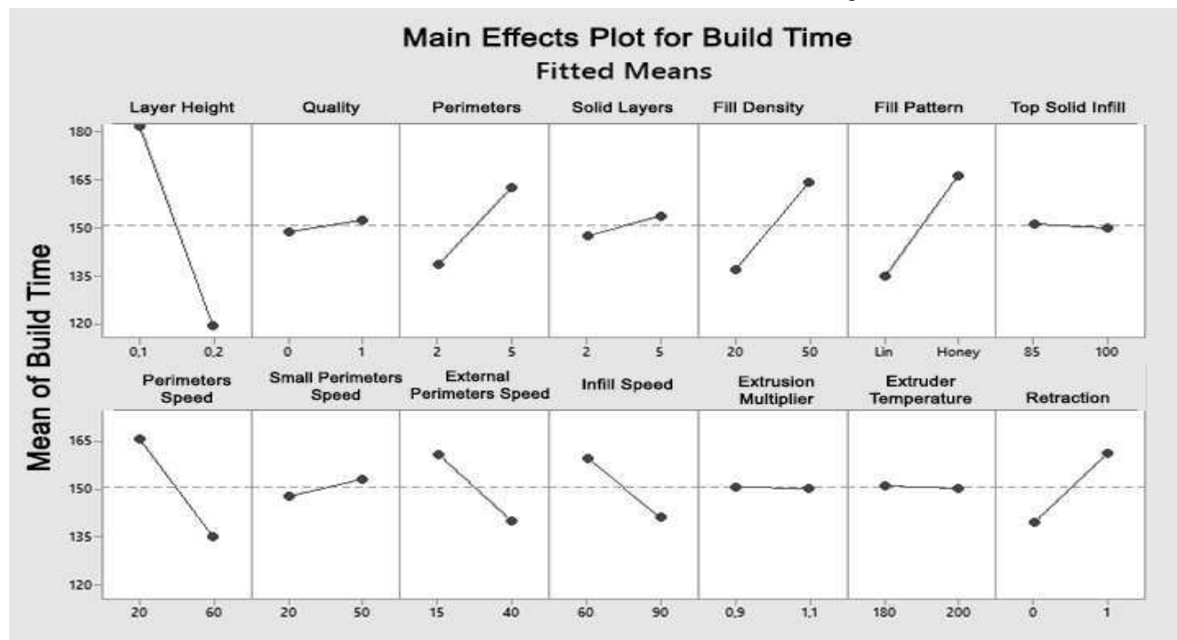
Fig. 3 Main Effects plot for Build Time.
